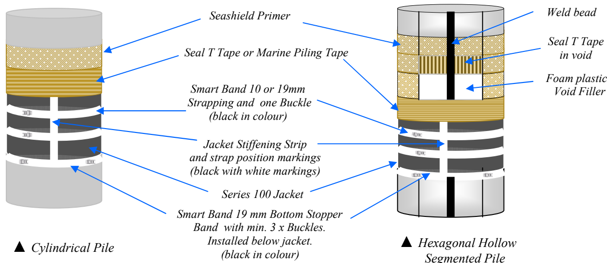
Figure 5. Illustrated examples of the Series 100 System on various piles
