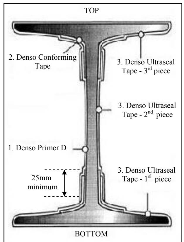
▼ Fig 5. Cross section diagram highlighting the correct sequence for applying the primer and tapes to an RSJ beam.
