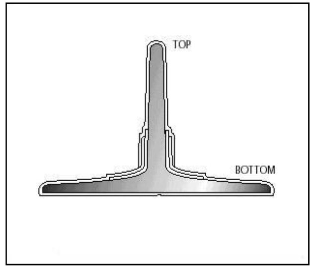
◀ Fig 6. The correct tape configuration for steel channels
