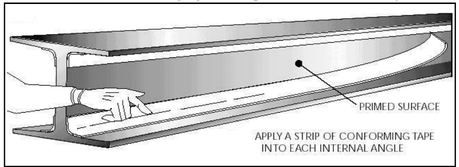
▲ Fig 2. Application and positioning of Conforming tape on Rolled Steel Joist (RSJ) beams.
