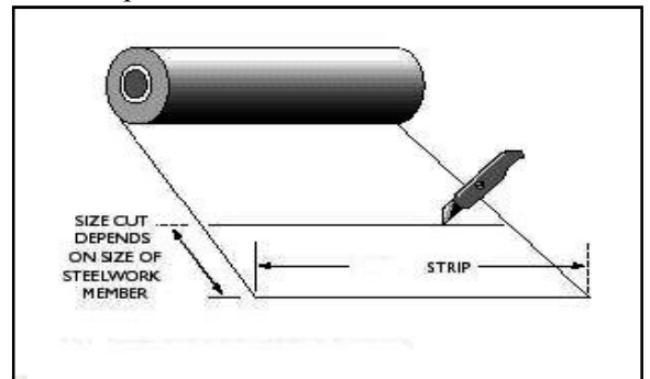
▲ Fig 4. Unrolling and preparing a strip of Ultraseal
