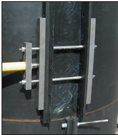
1. A new hydraulic clamp now rapidly pulls the jacket seams together.
